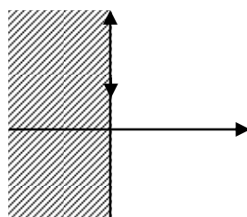
\text{Re } z > 0
