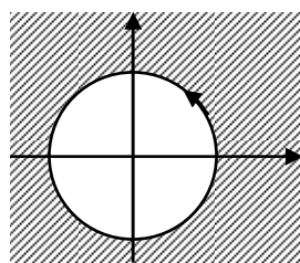
|z| < R
