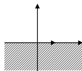
\text{Im } z > 0
